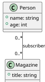
Figure 65: Example of association in UML class diagrams
